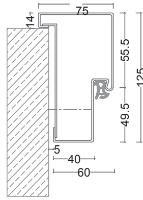
Architrave: 125x60x75mm
