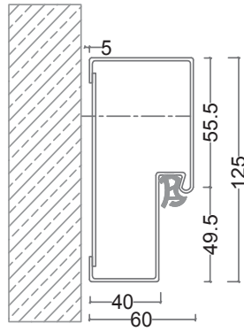
Standard: 125x60mm
